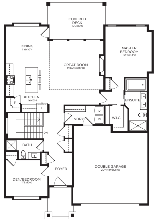
MAIN FLOOR PLAN 1,464 SQ.FT.
