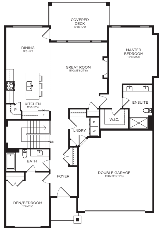
MAIN FLOOR PLAN 1,550 SQ.FT.
